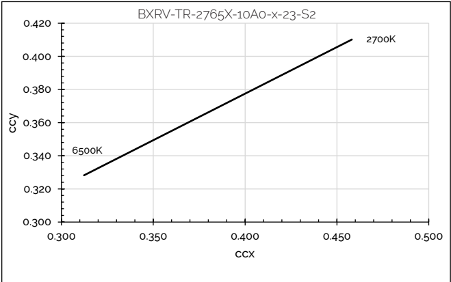
Figure 25: CCT Tuning Range, Tc=85°C
