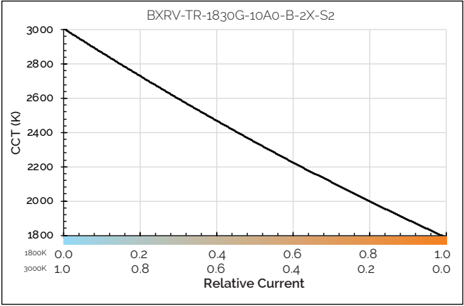
Figure 20: CCT vs. Relative Current, Tc=85°C
