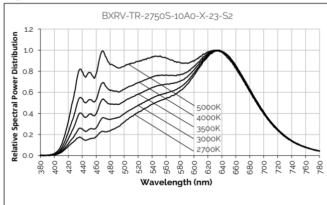
Figure 30: 2700K - 5000K with Thrive
