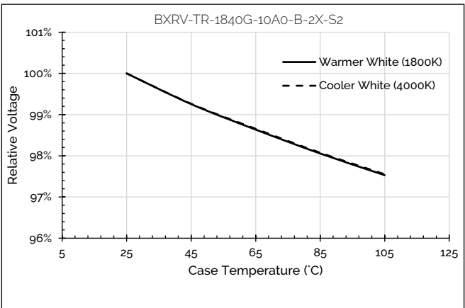
Figure 17: Relative Voltage vs. Case Temperature
