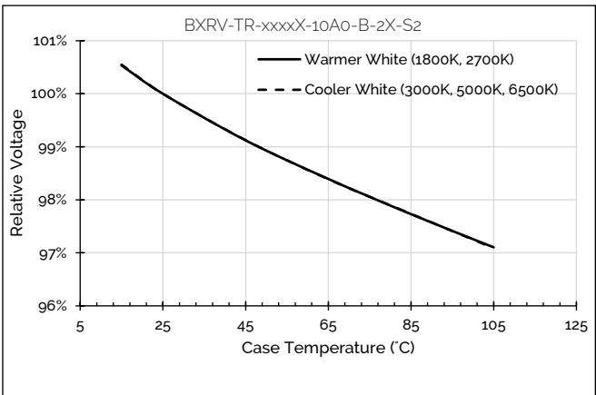
Figure 16: Relative Voltage vs. Case Temperature
