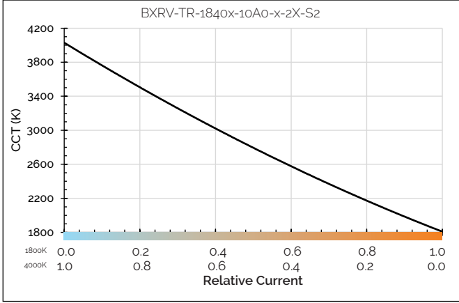
Figure 21: CCT vs. Relative Current, Tc=85°C
