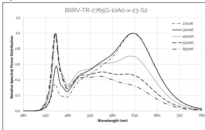
Figure 34: 2700K - 6500K with 90 CRI
