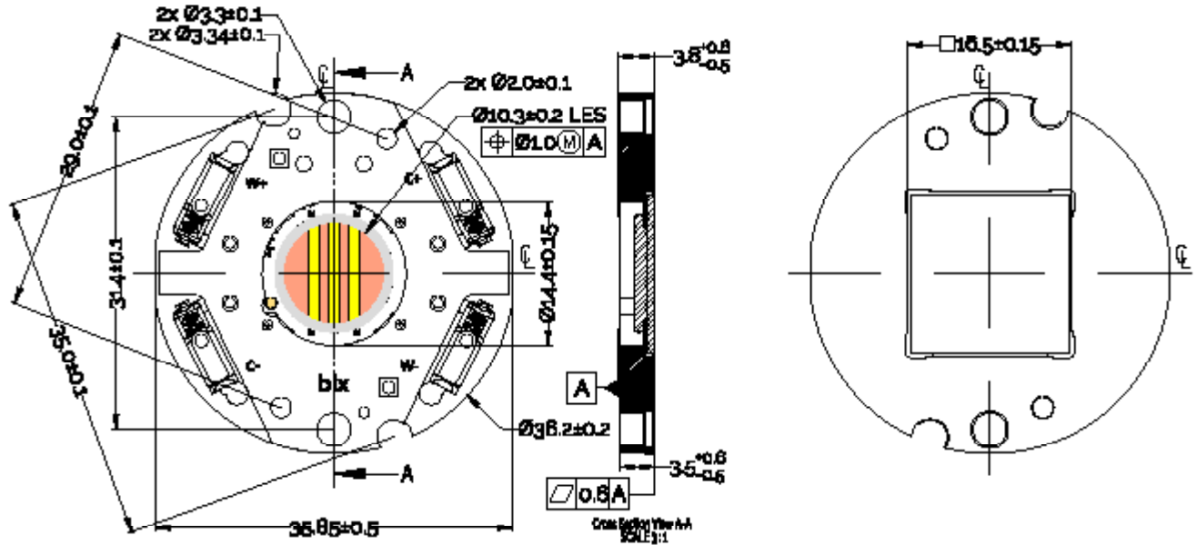
Figure 37: Mechanical Drawing Specifications
