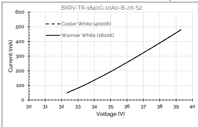
Figure 8: Forward Voltage vs. Forward Current, T_c=25^\circ\text{C}
