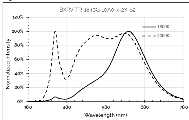
Figure 36: 1800K - 4000K with 90 CRI
