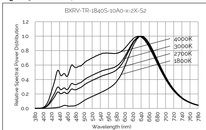
Figure 32: 1800K - 4000K with Thrive
