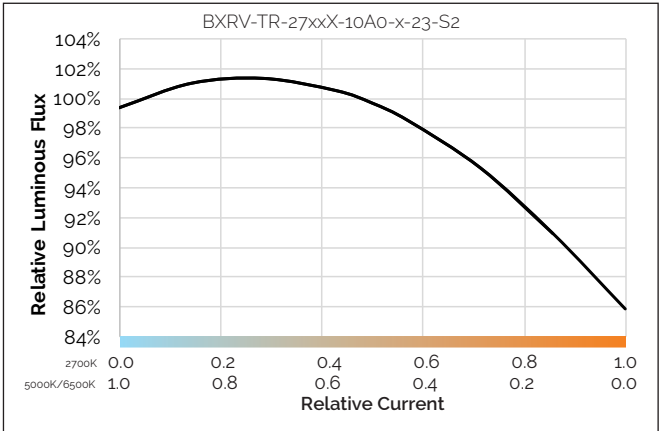
Figure 22: Relative Flux vs. Relative Current
