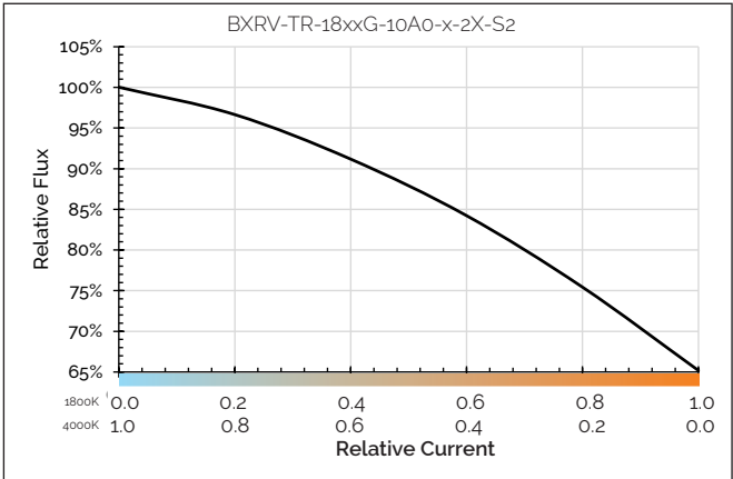
Figure 23: Relative Flux vs. Relative Current
