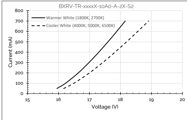
Figure 6: Forward Voltage vs. Forward Current, T_c=25^\circ\text{C}
