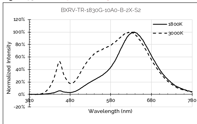
Figure 35: 1800K - 3000K with 90 CRI
