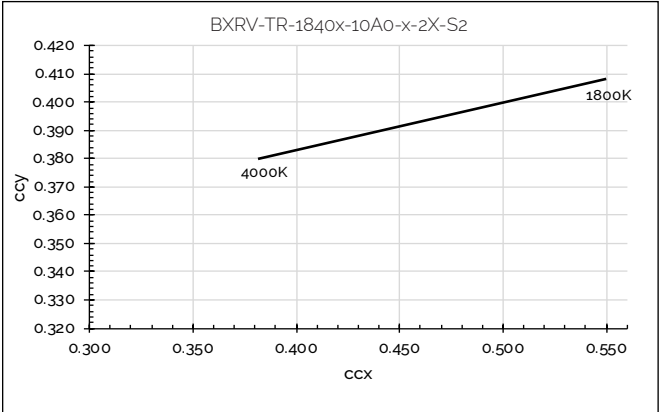
Figure 27: CCT Tuning Range, Tc=85°C
