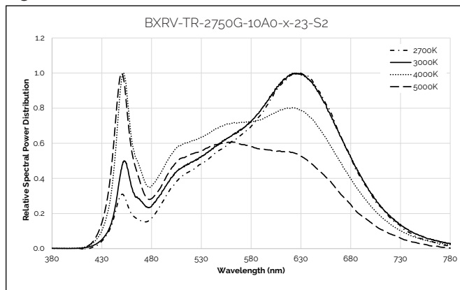
Figure 33: 2700K - 5000K with 90 CRI
