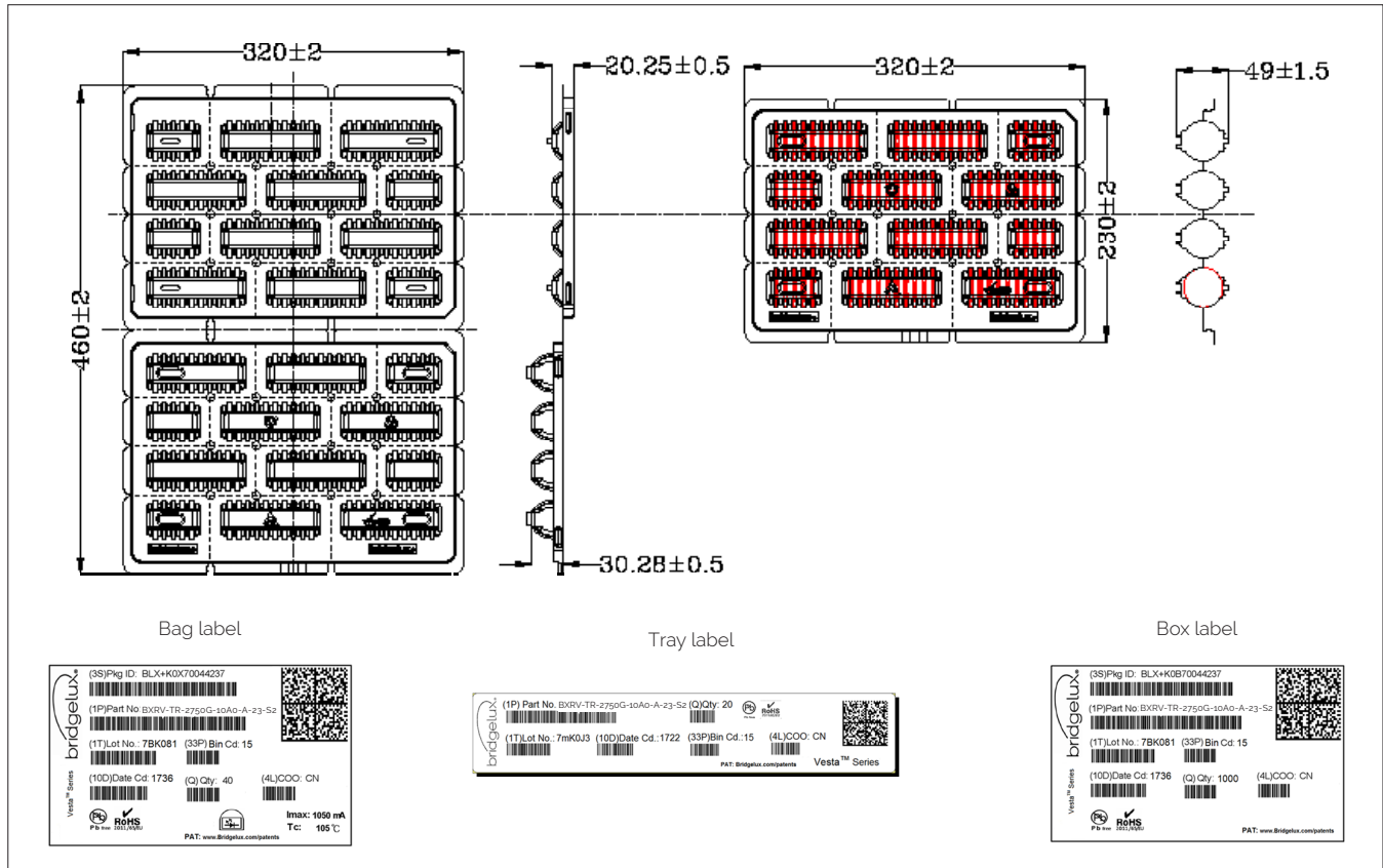
Figure 40: Packaging Specifications
