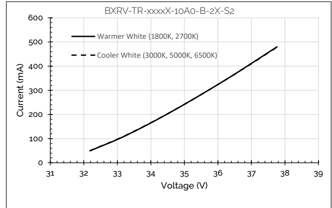
Figure 7: Forward Voltage vs. Forward Current, T_c=25^\circ\text{C}
