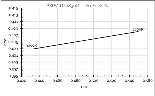
Figure 26: CCT Tuning Range, Tc=85°C
