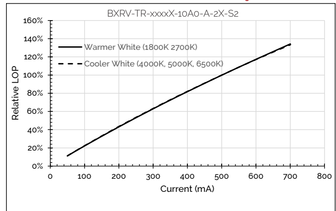
Figure 9: Relative Flux vs. Drive Current, T_c=25^\circ\text{C}
