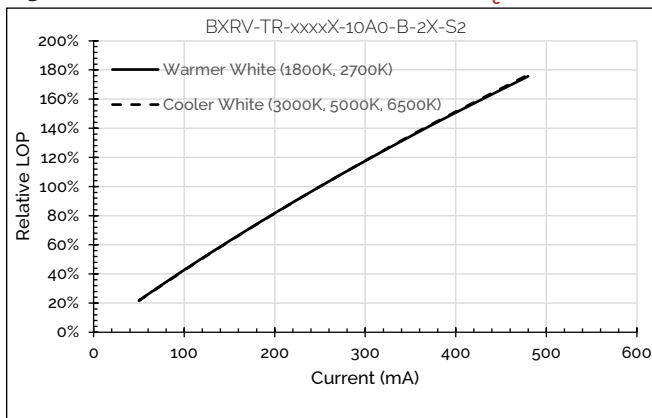
Figure 10: Relative Flux vs. Drive Current, T_c=25^\circ\text{C}
